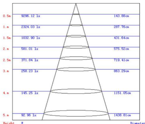
Lux-Distance Curve
