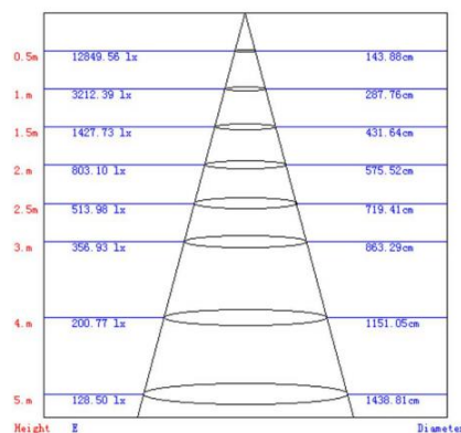
Lux-Distance Curve
